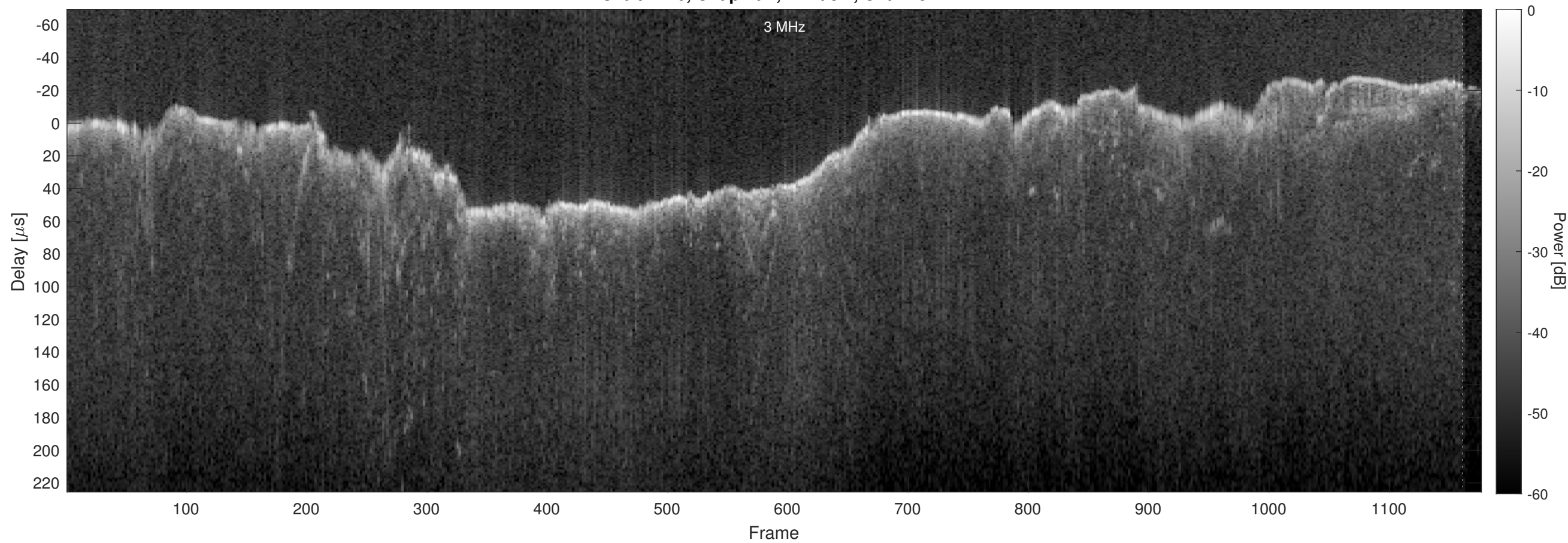
Orbit 2776, Chapman, Window, Channel 2
