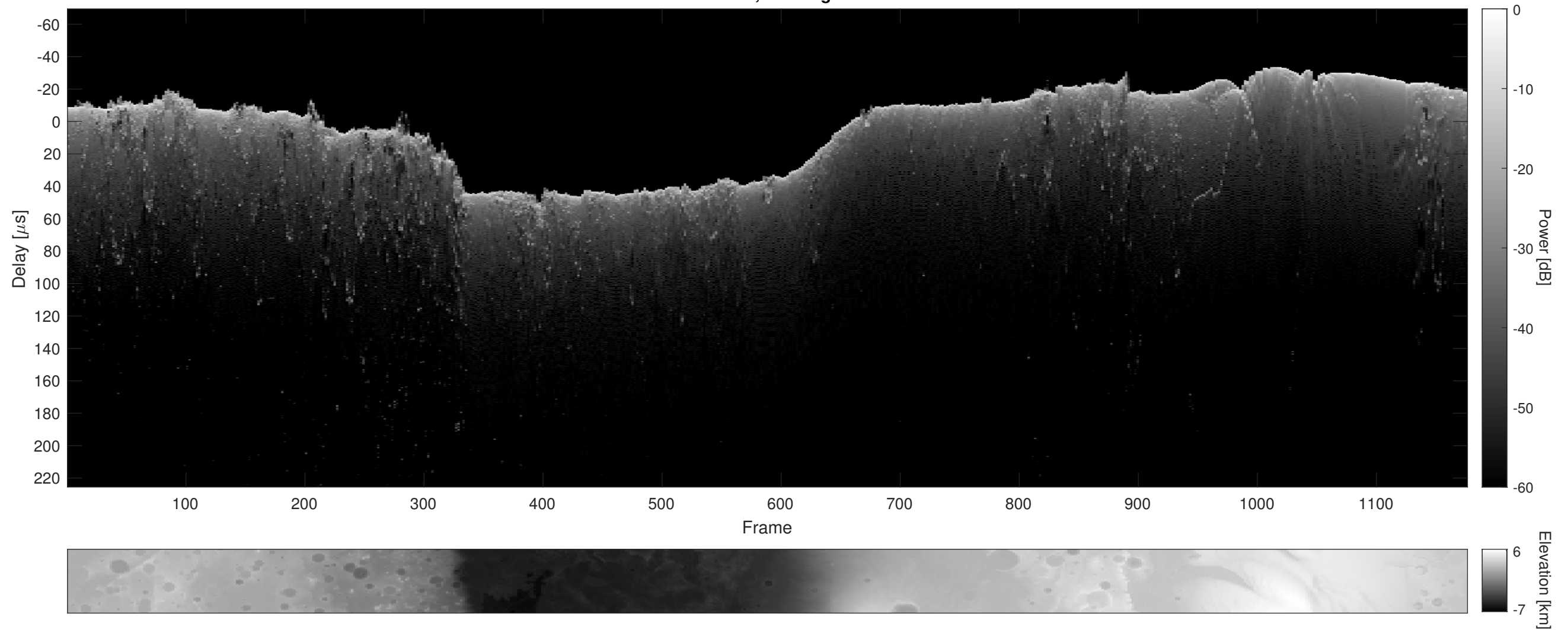
Orbit 2776, Cluttergram
