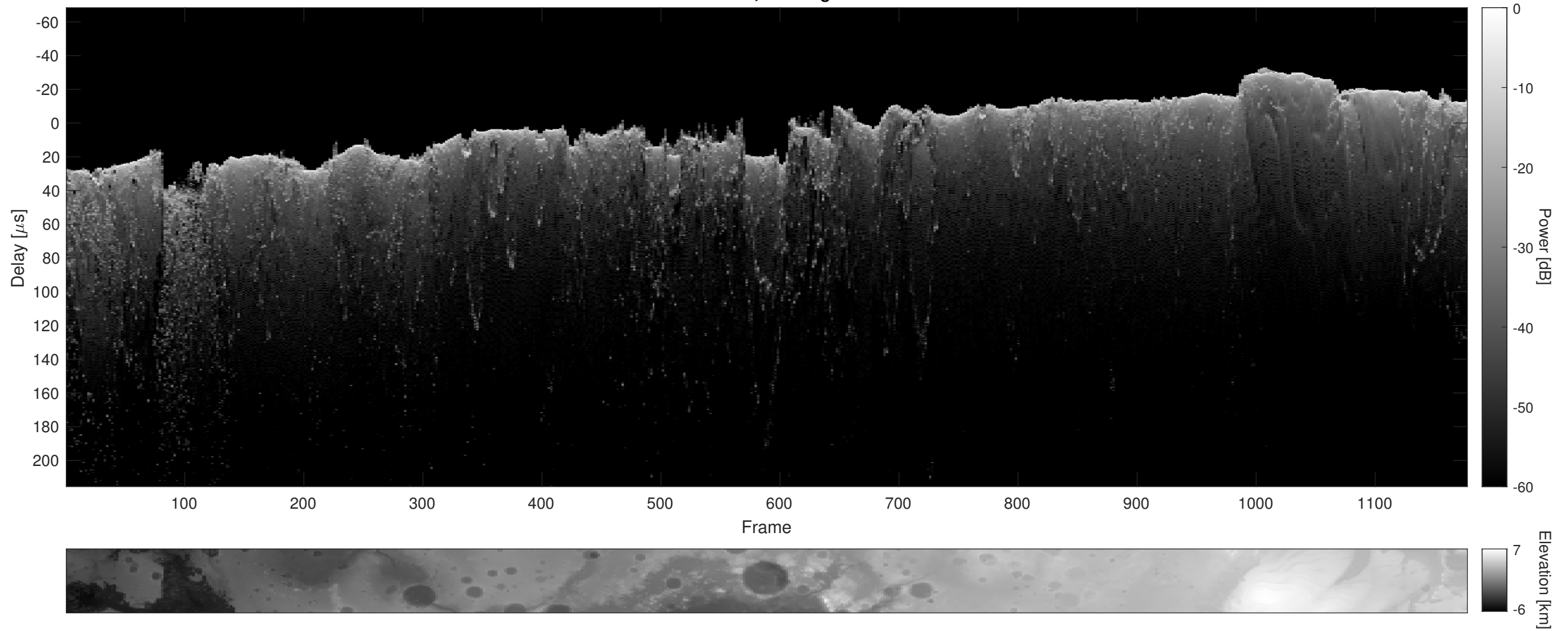
Orbit 2777, Cluttergram
