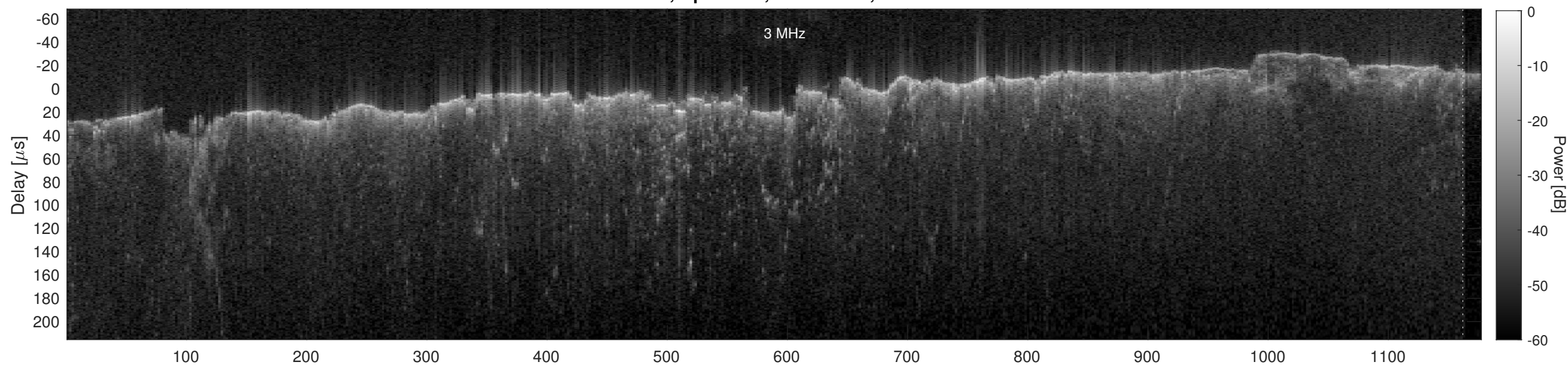
Orbit 2777, Cluttergram
