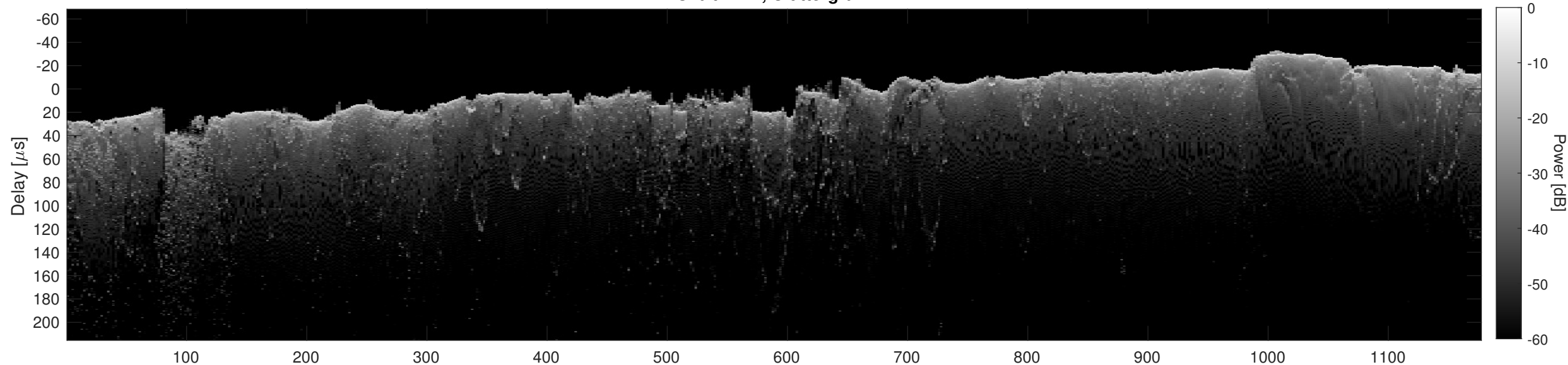
Orbit 2777, Cluttergram
