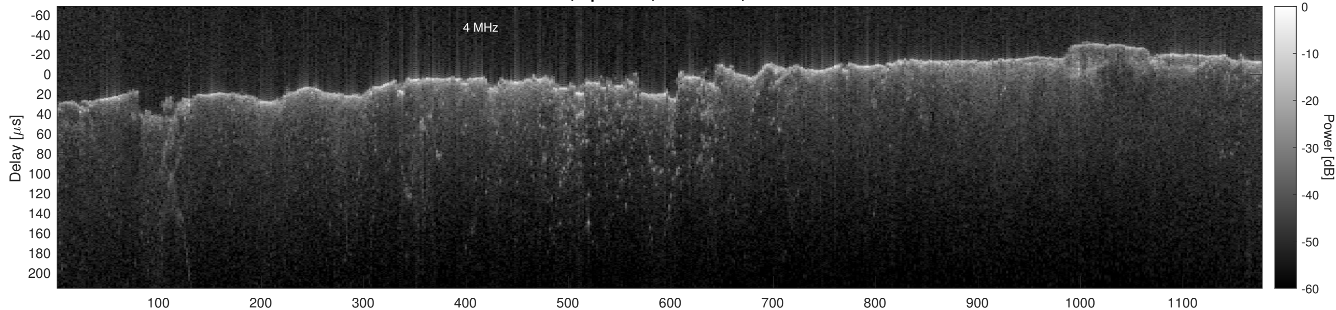
Orbit 2777, Optimized, No Window, Channel 2
