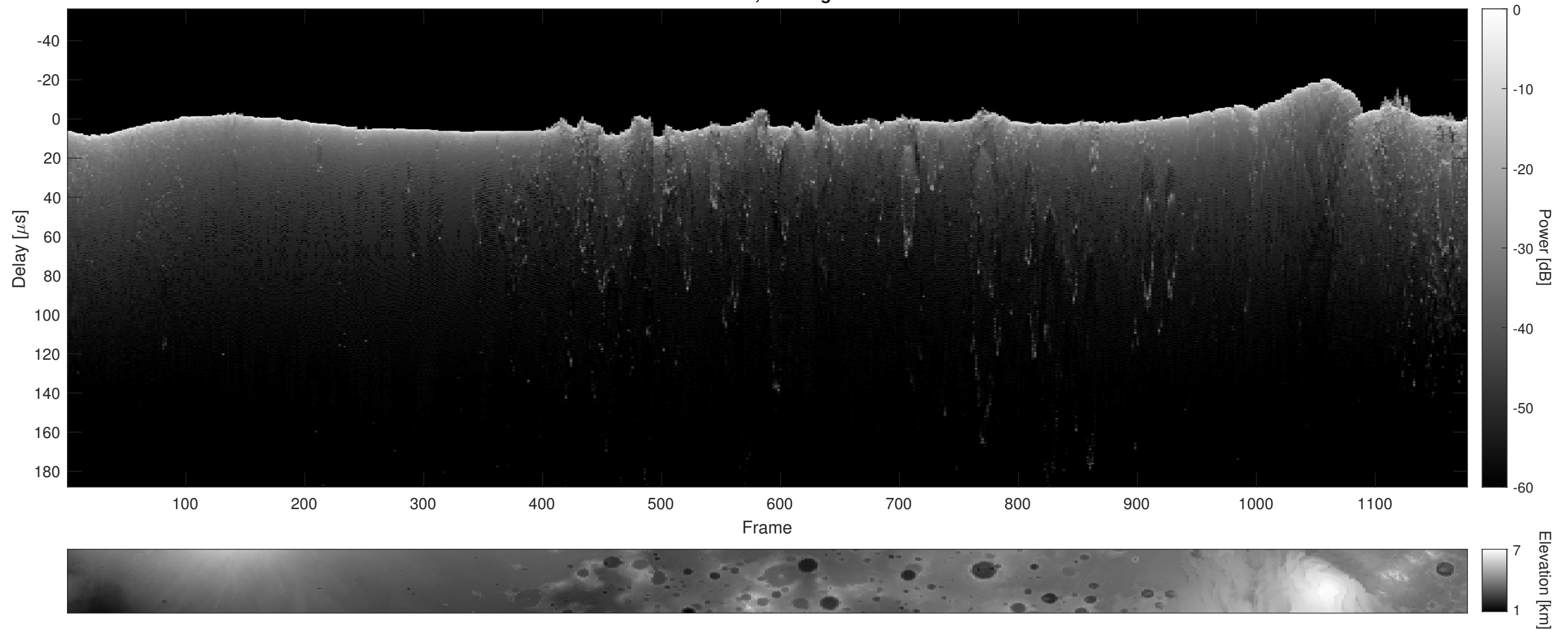
Orbit 2778, Cluttergram
