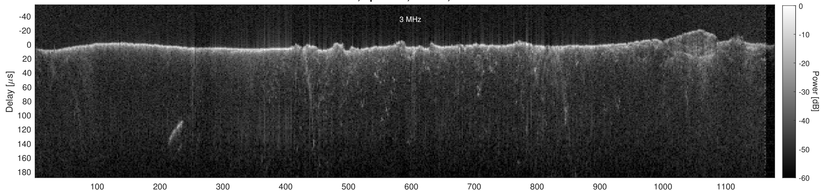
Orbit 2778, Cluttergram
