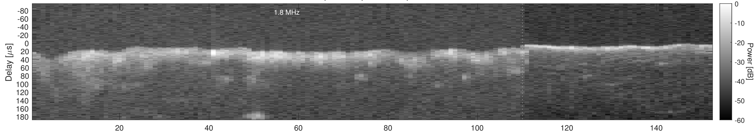
Orbit 2780, Window, Channel 2, Chapman
