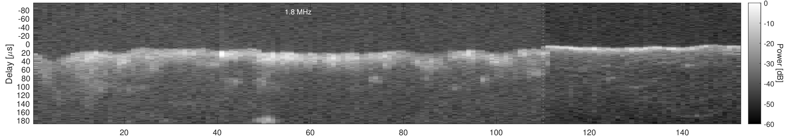
Orbit 2780, Window, Channel 2, Optimized
