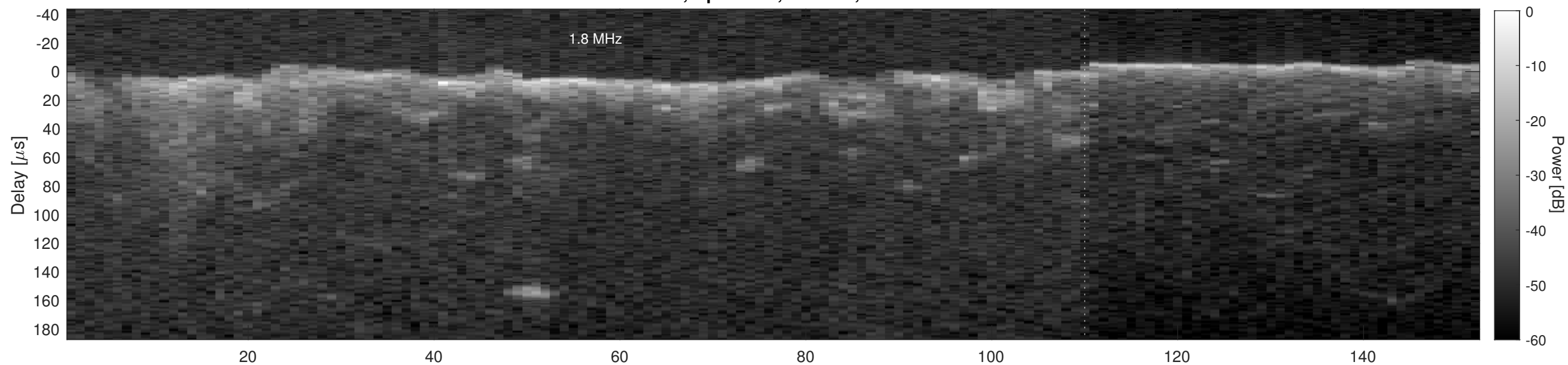
Orbit 2780, Cluttergram
