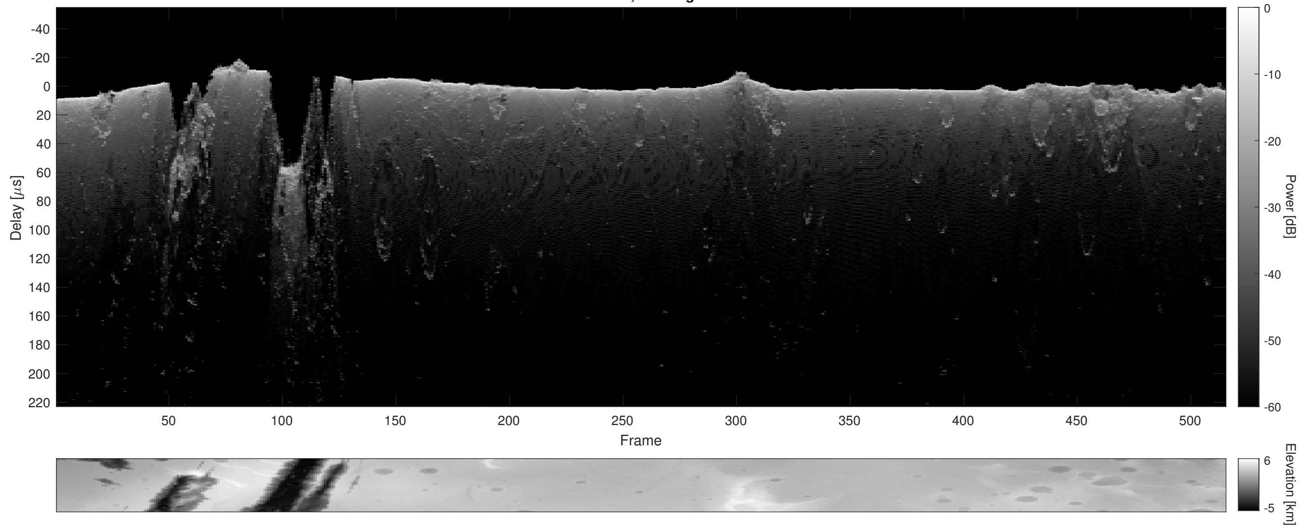
Orbit 2781, Cluttergram
