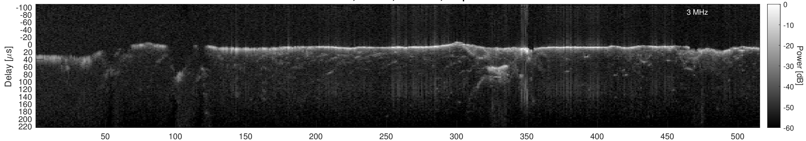
Orbit 2781, Window, Channel 2, Optimized
