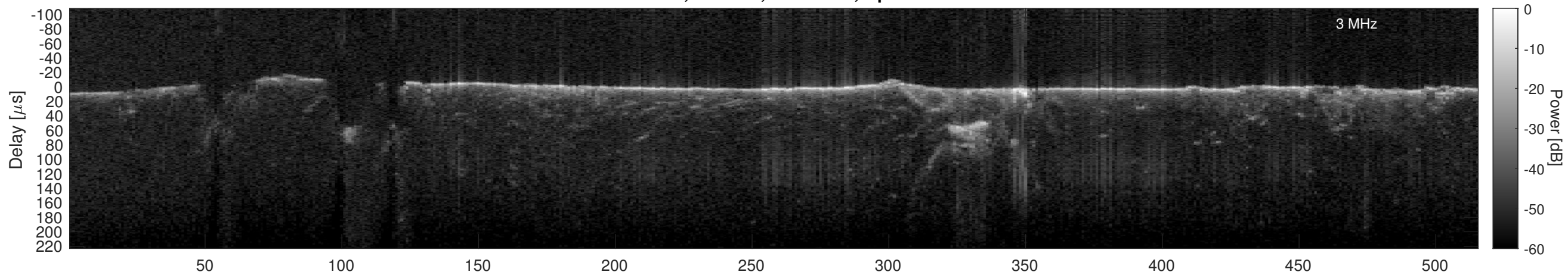
Orbit 2781, Cluttergram
