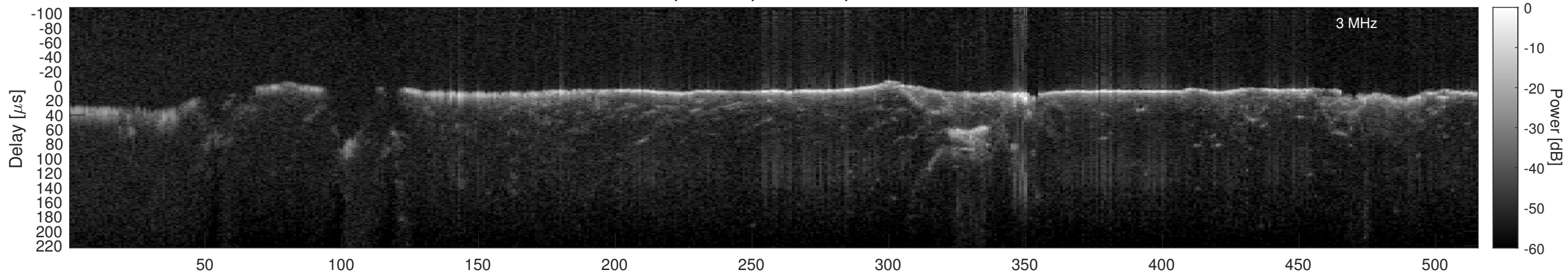
Orbit 2781, Window, Channel 2, Chapman
