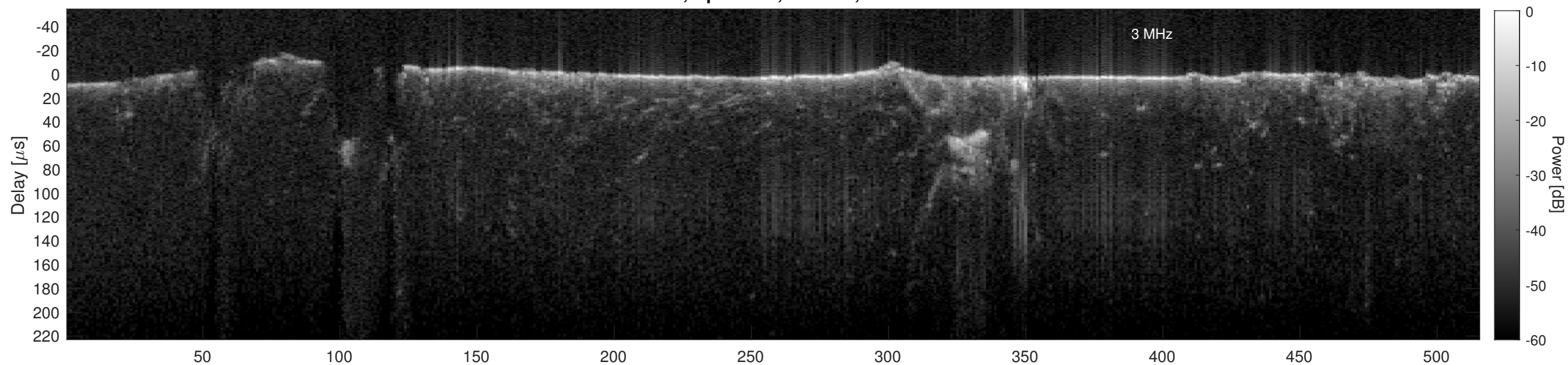
Orbit 2781, Cluttergram
