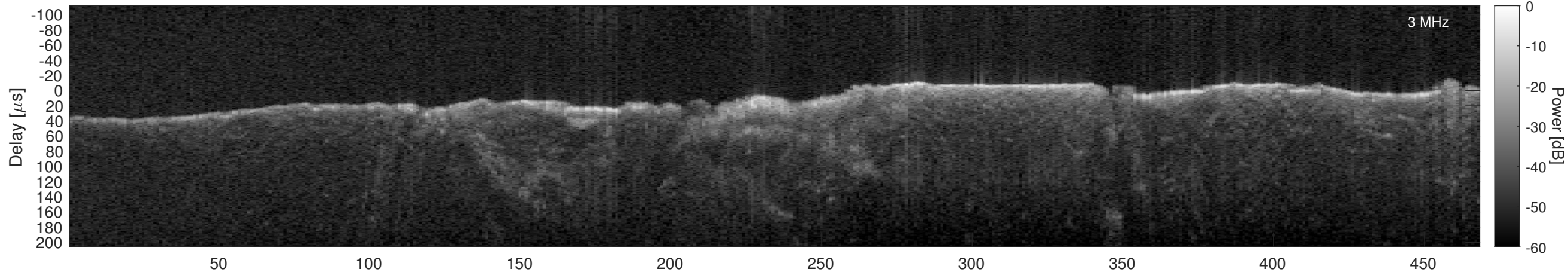
Orbit 2782, Window, Channel 2, Chapman
