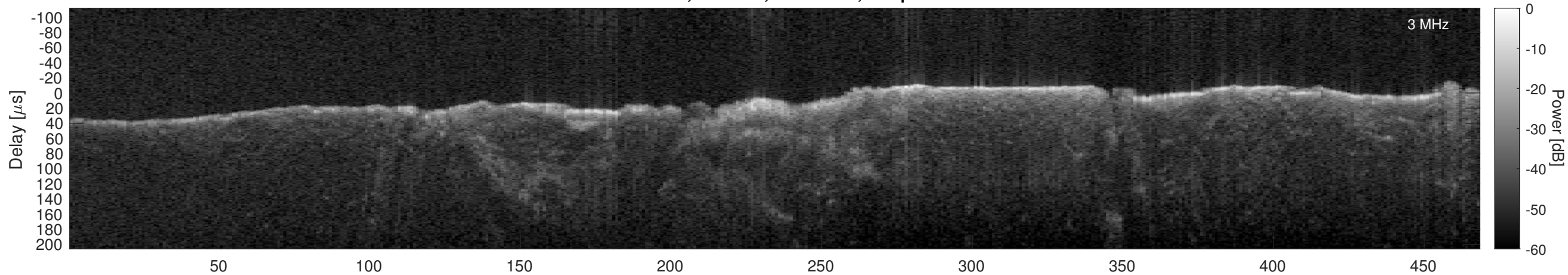
Orbit 2782, Window, Channel 2, Optimized
