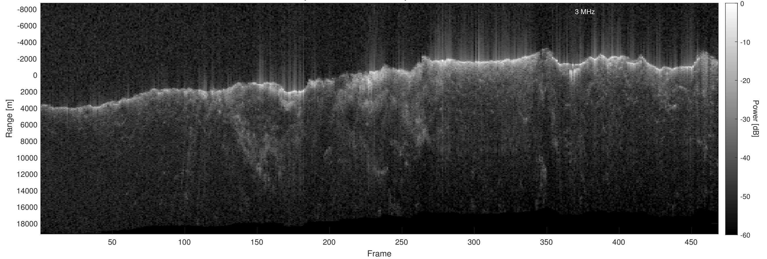
Orbit 2782, Optimized, No Window, Depth-Corrected, Channel 2
