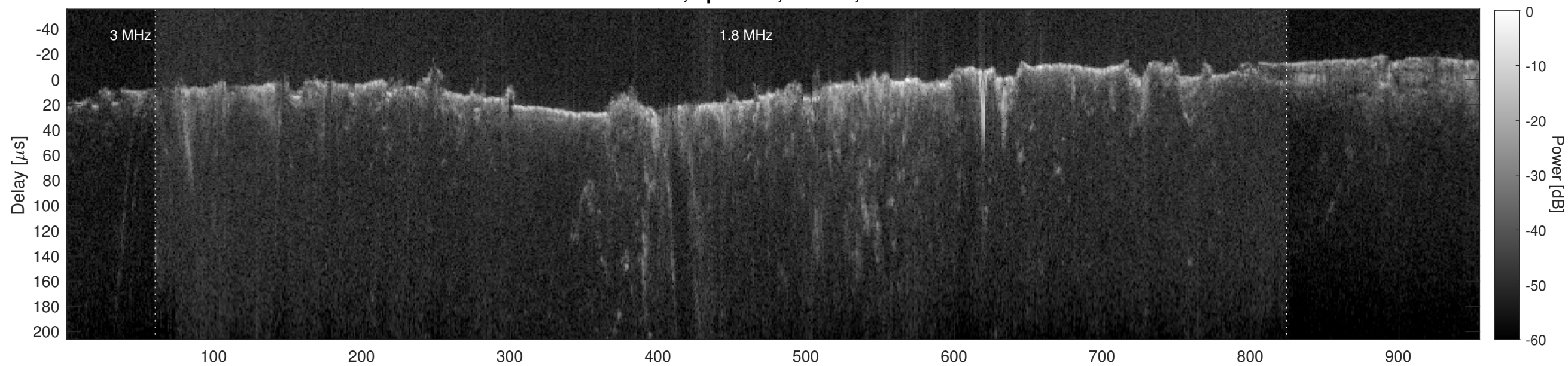
Orbit 2783, Cluttergram
