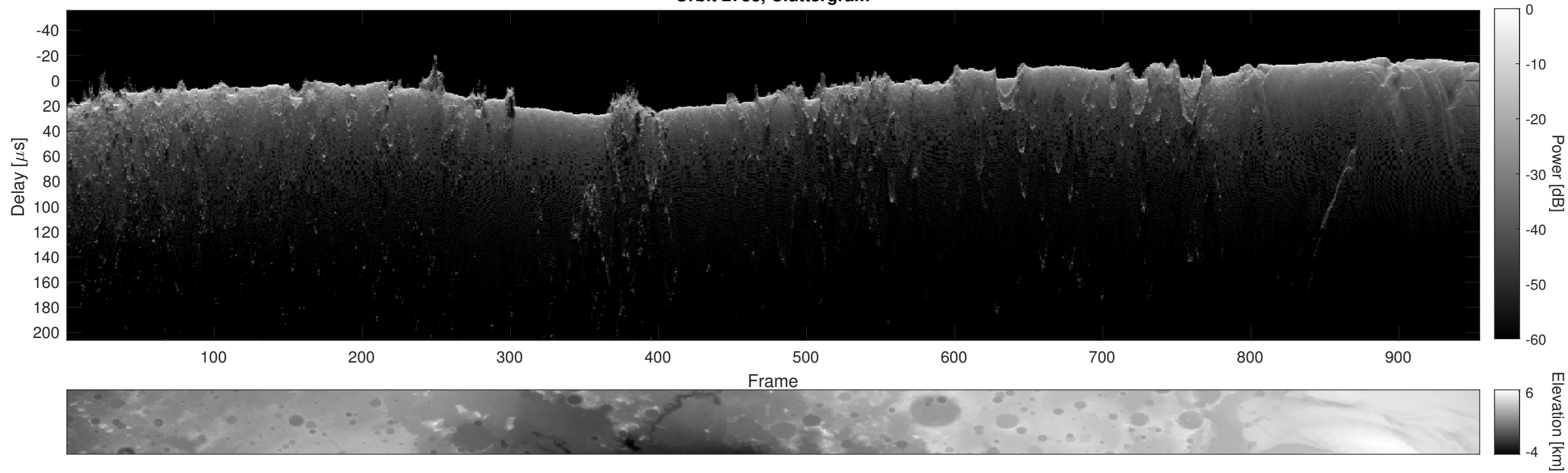
Orbit 2783, Cluttergram
