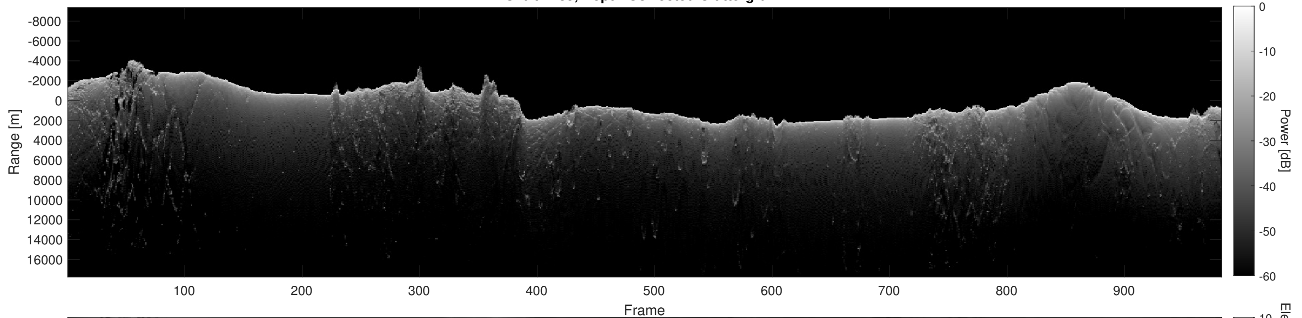
Orbit 2785, Depth-Corrected Cluttergram
