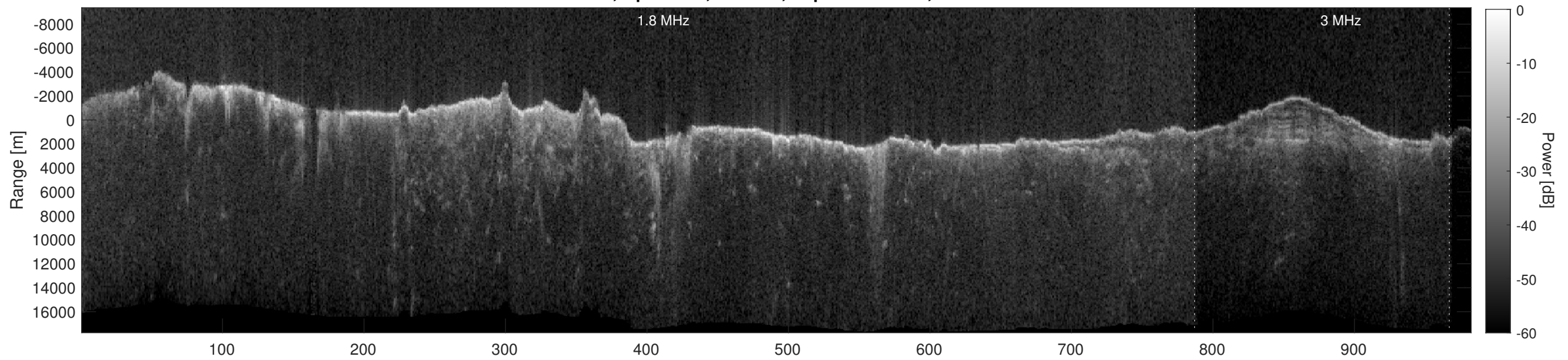
Orbit 2785, Depth-Corrected Cluttergram
