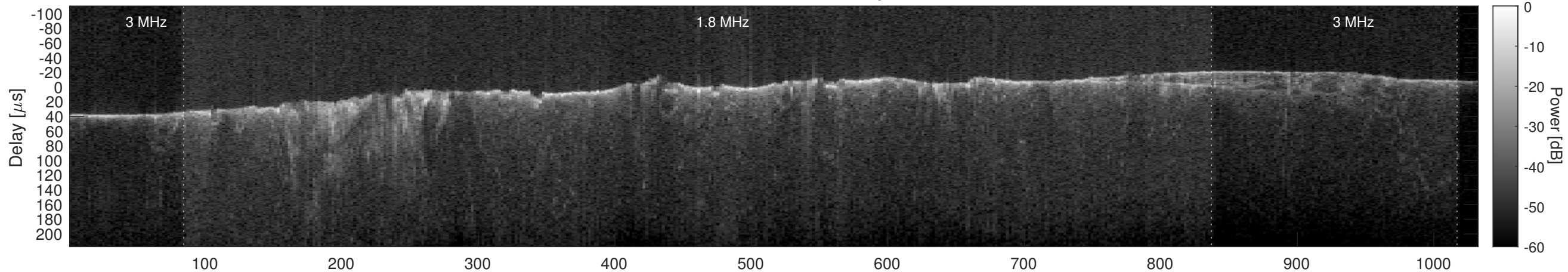
Orbit 2786, Cluttergram
