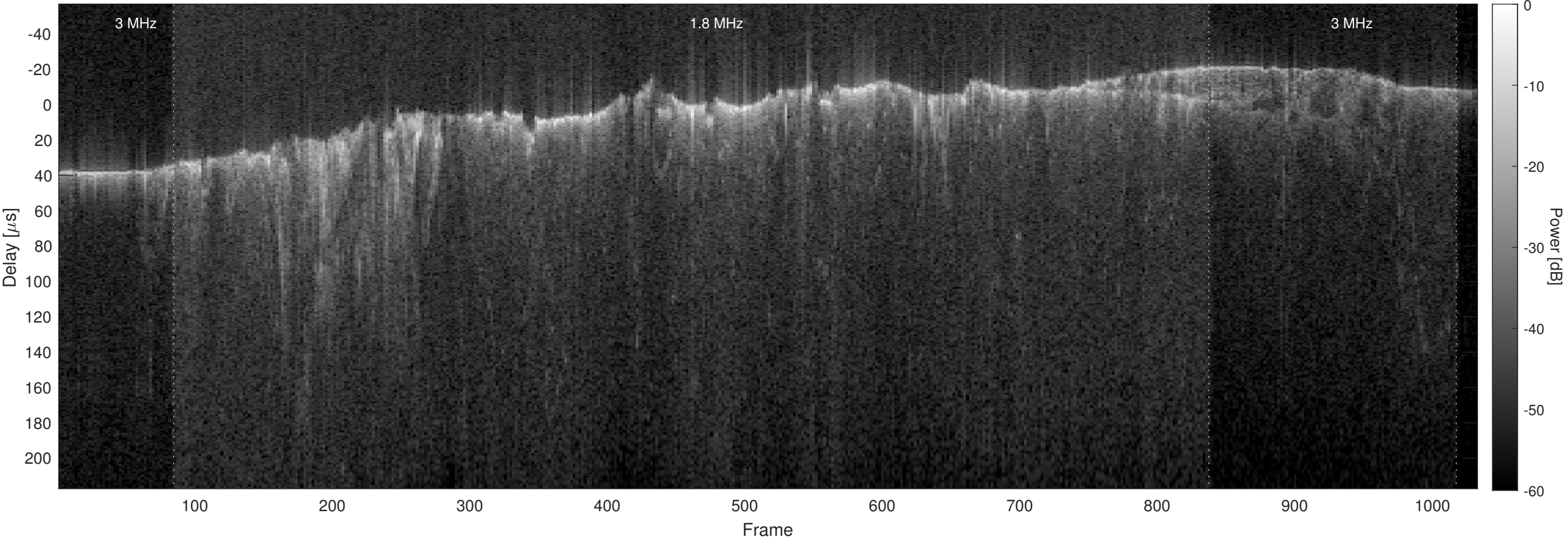
Orbit 2786, Optimized, No Window, Channel 2
