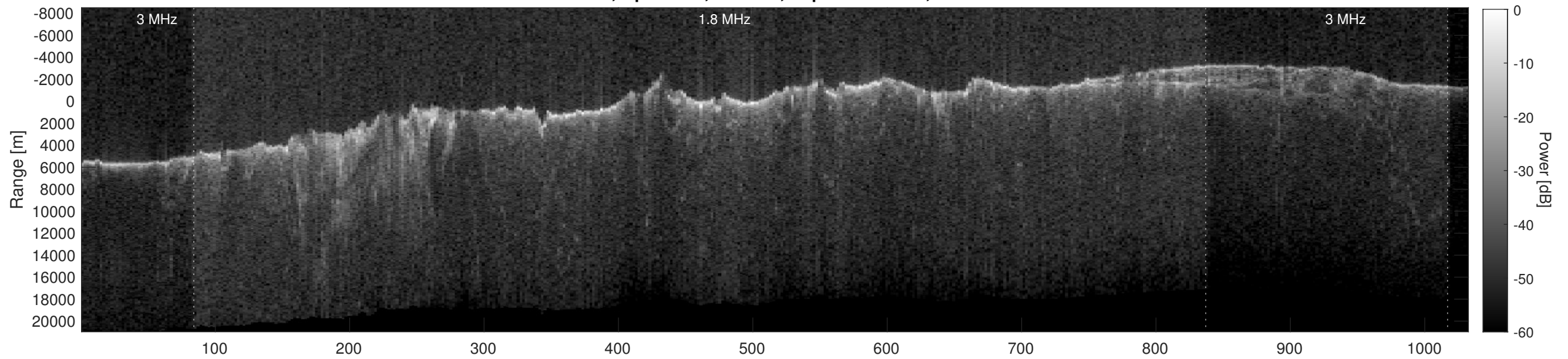
Orbit 2786, Depth-Corrected Cluttergram
