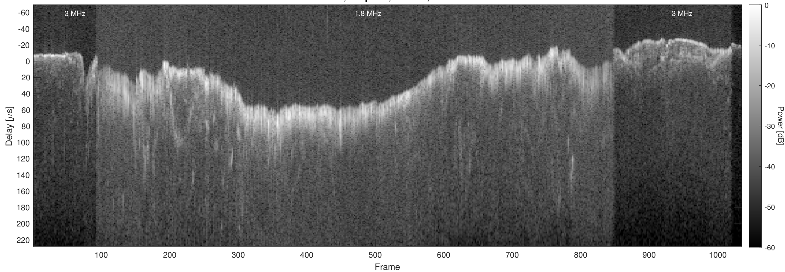
Orbit 2787, Chapman, Window, Channel 2
