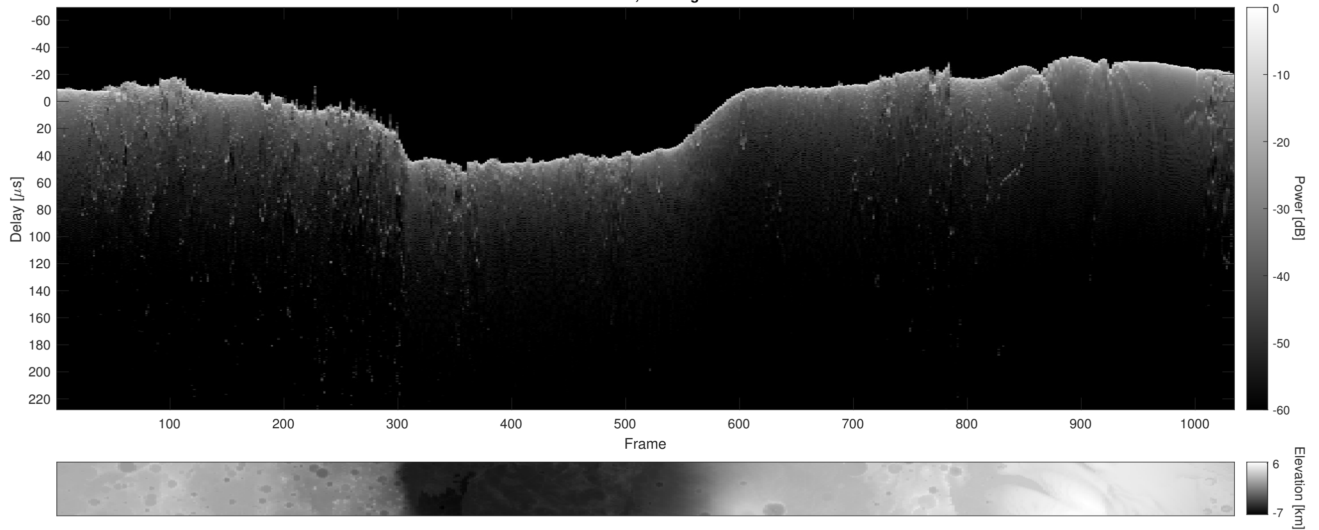
Orbit 2787, Cluttergram
