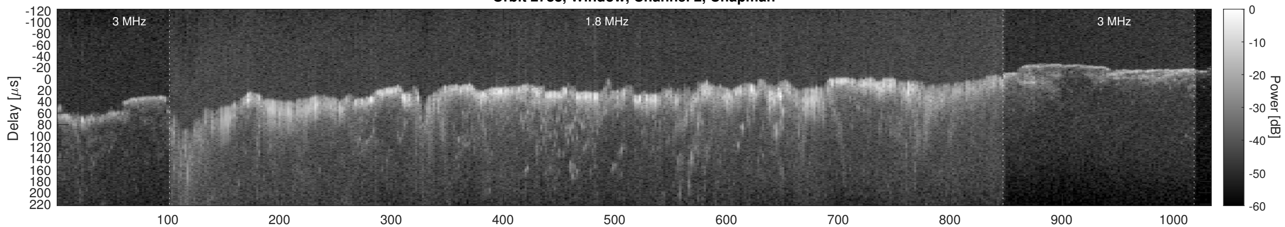
Orbit 2788, Window, Channel 2, Optimized
