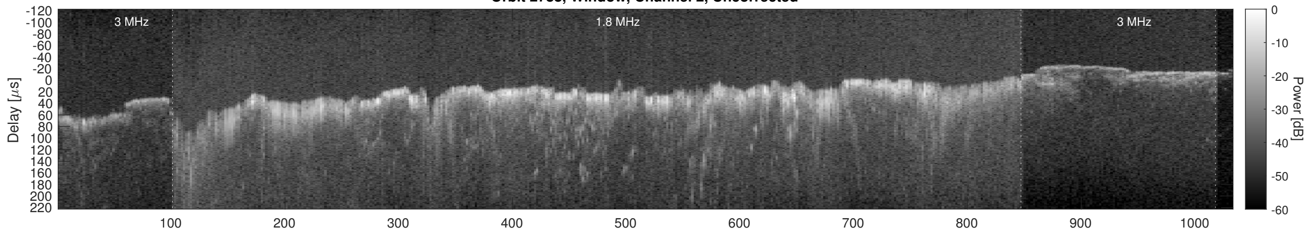
Orbit 2788, Window, Channel 2, Chapman
