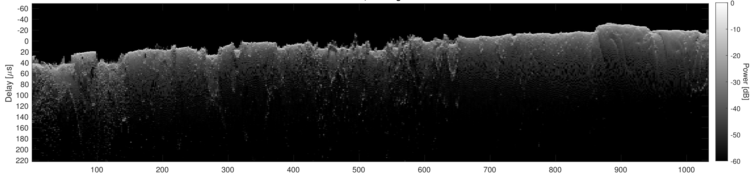
Orbit 2788, Cluttergram
