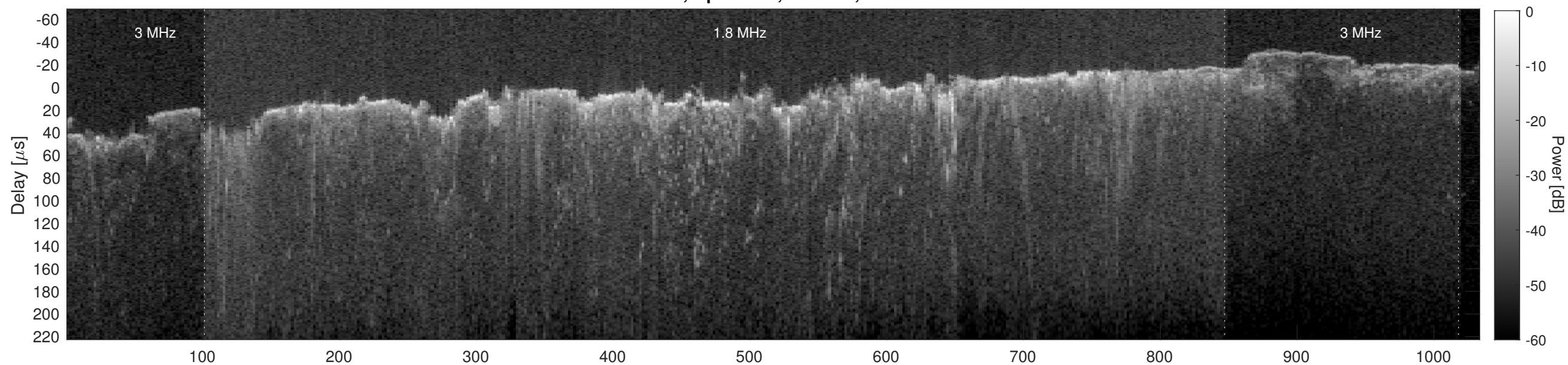
Orbit 2788, Cluttergram
