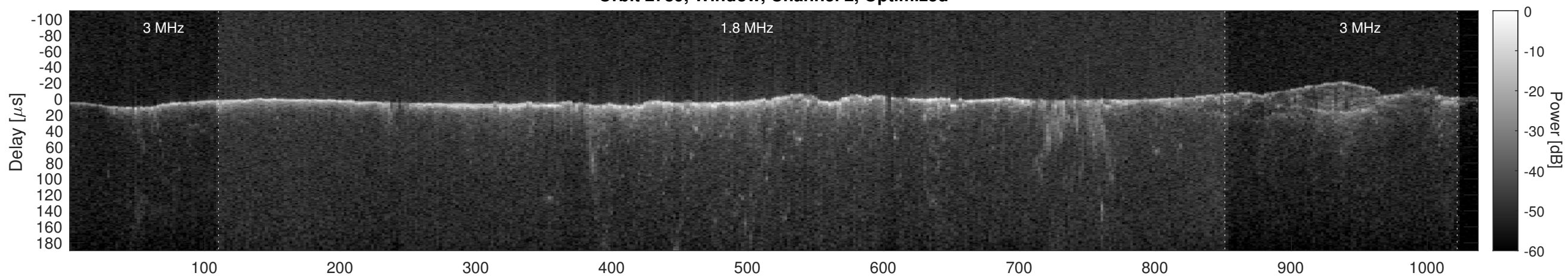
Orbit 2789, Cluttergram
