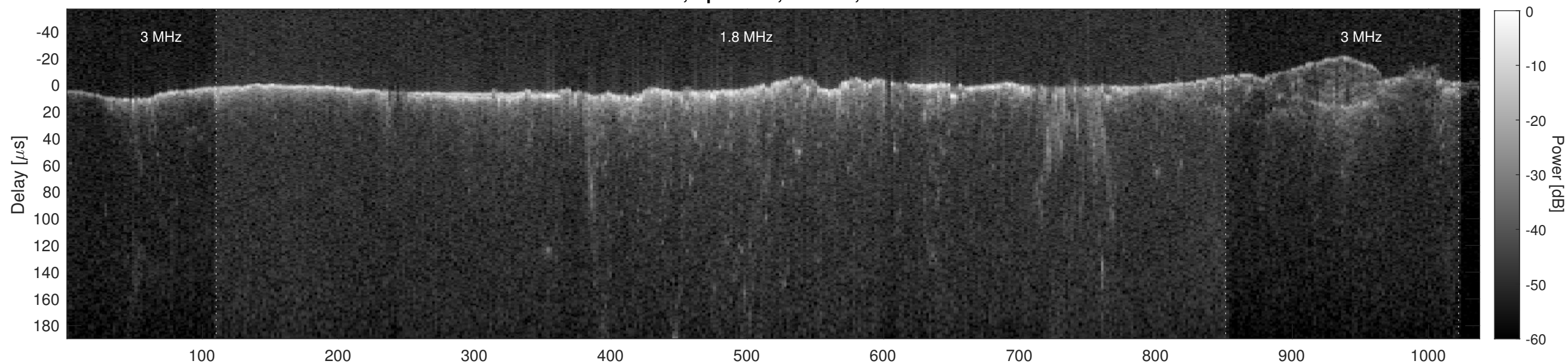
Orbit 2789, Cluttergram
