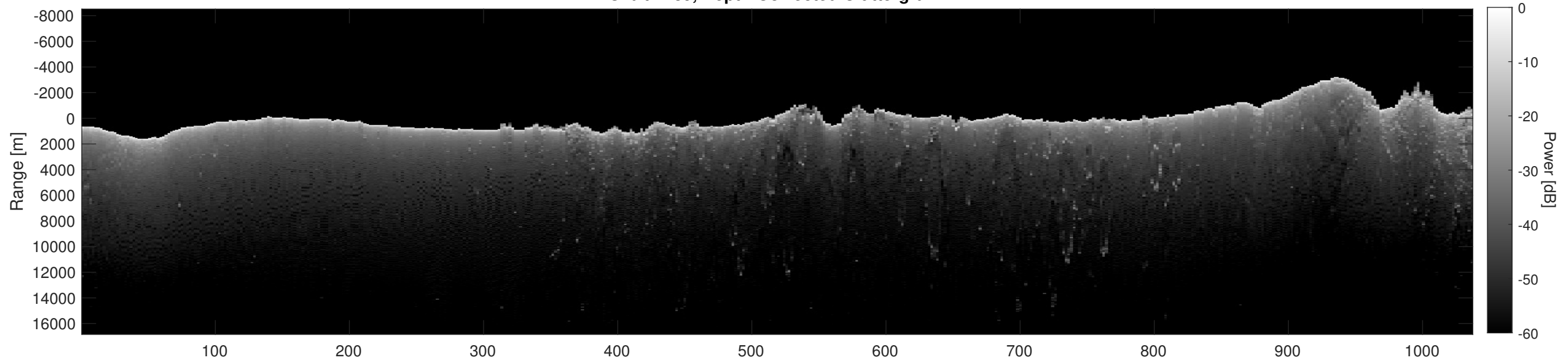
Orbit 2789, Depth-Corrected Cluttergram
