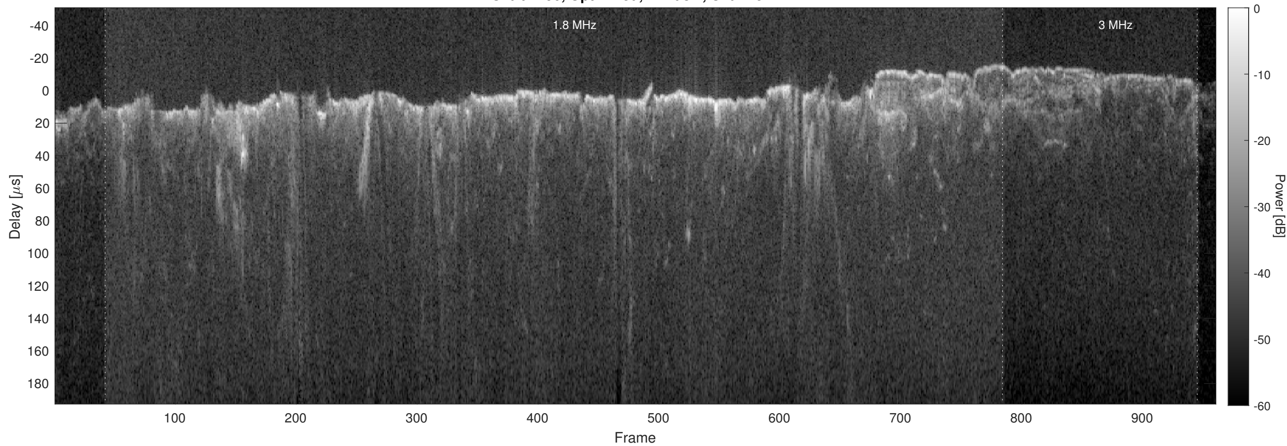
Orbit 2790, Optimized, Window, Channel 2
