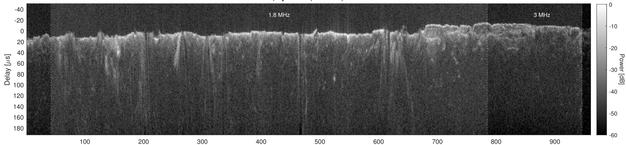
Orbit 2790, Cluttergram
