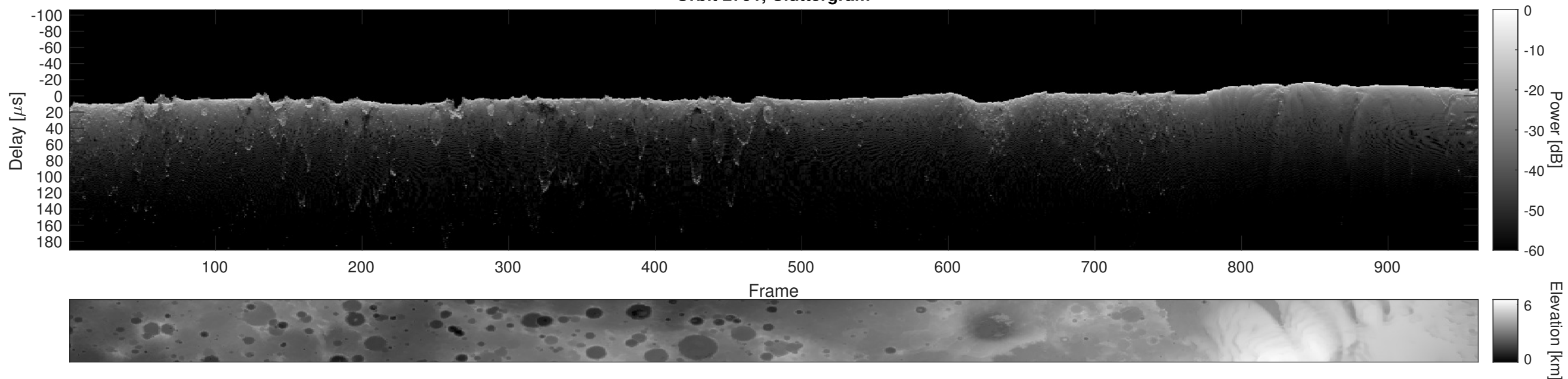
Orbit 2791, Cluttergram
