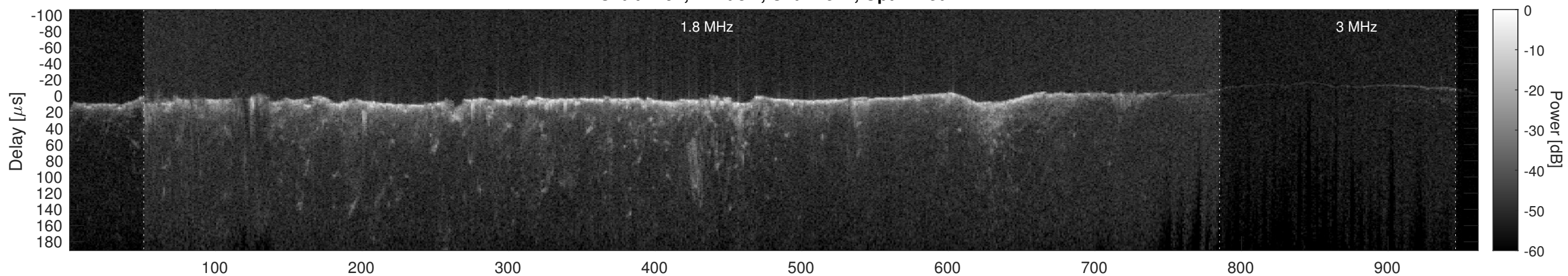
Orbit 2791, Cluttergram
