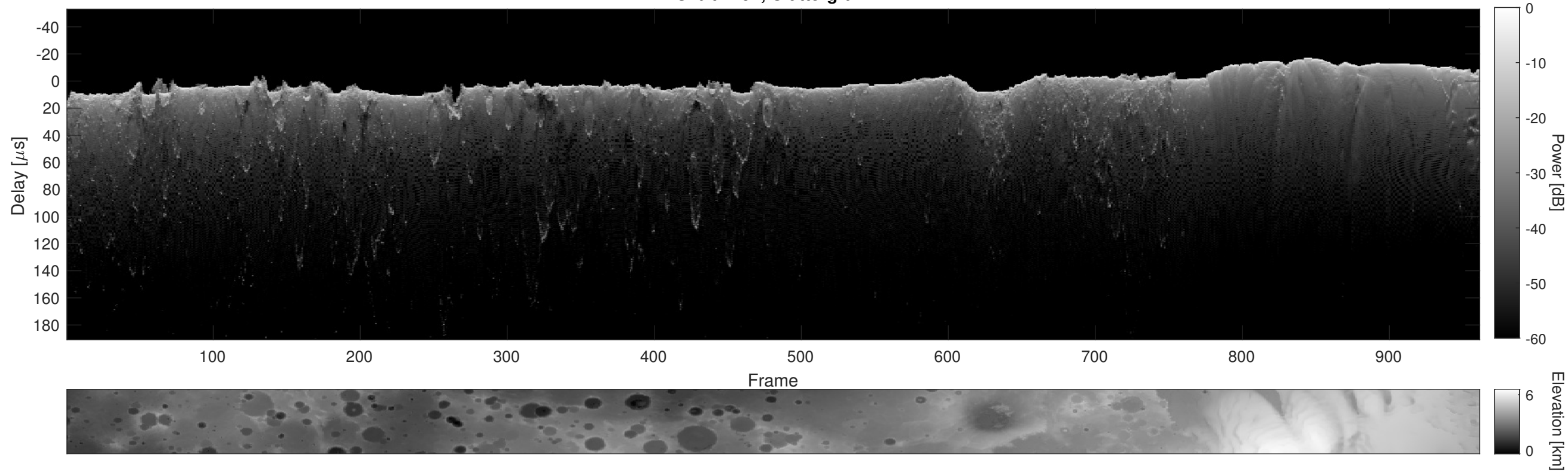
Orbit 2791, Cluttergram
