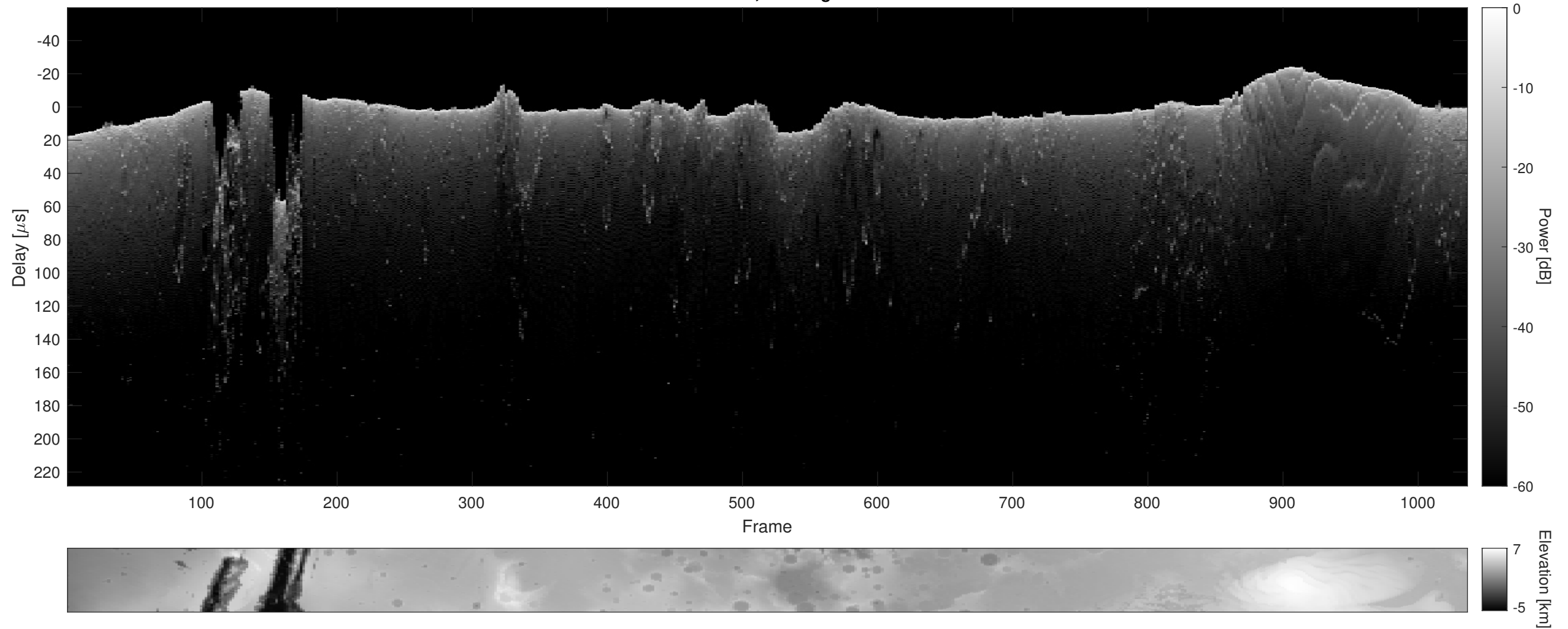
Orbit 2792, Cluttergram
