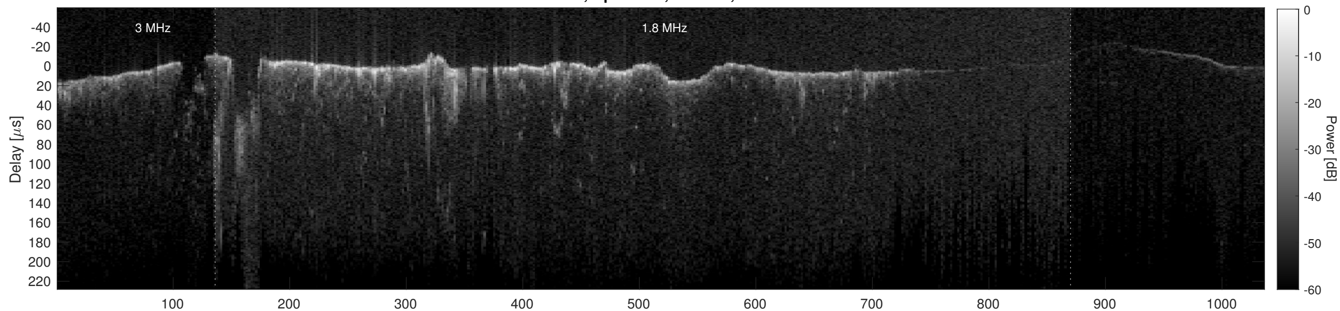
Orbit 2792, Cluttergram
