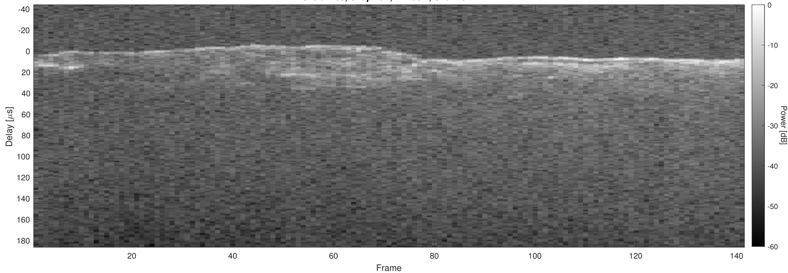
Orbit 2793, Chapman, Window, Channel 2
