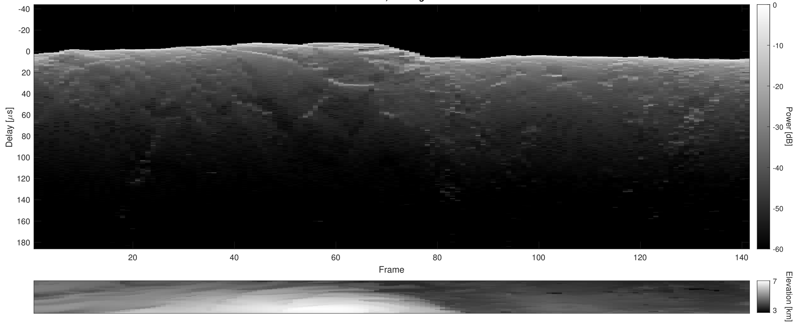
Orbit 2793, Cluttergram
