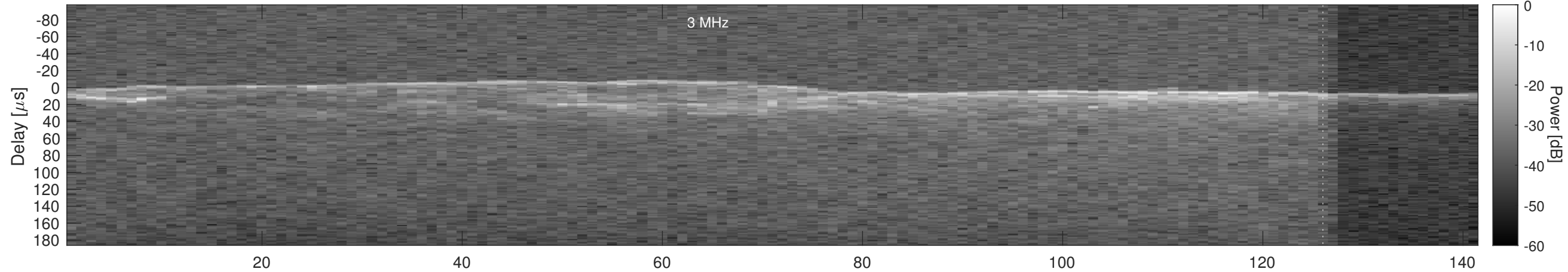
Orbit 2793, Cluttergram
