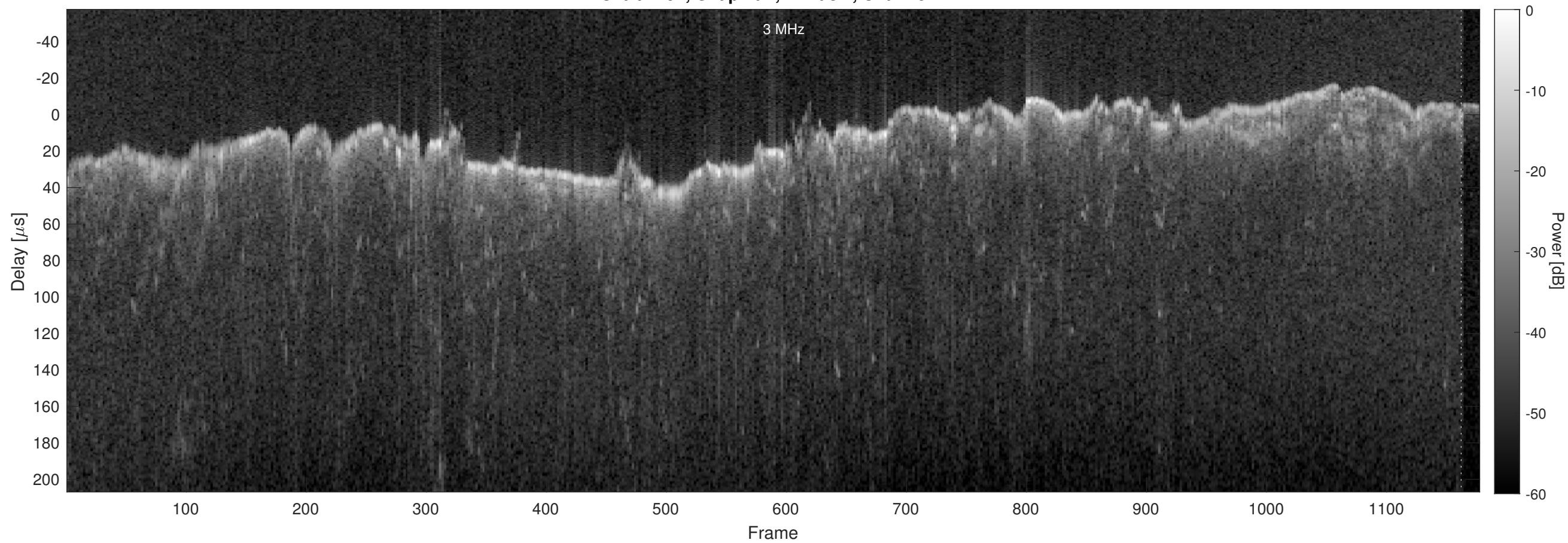
Orbit 2794, Chapman, Window, Channel 2
