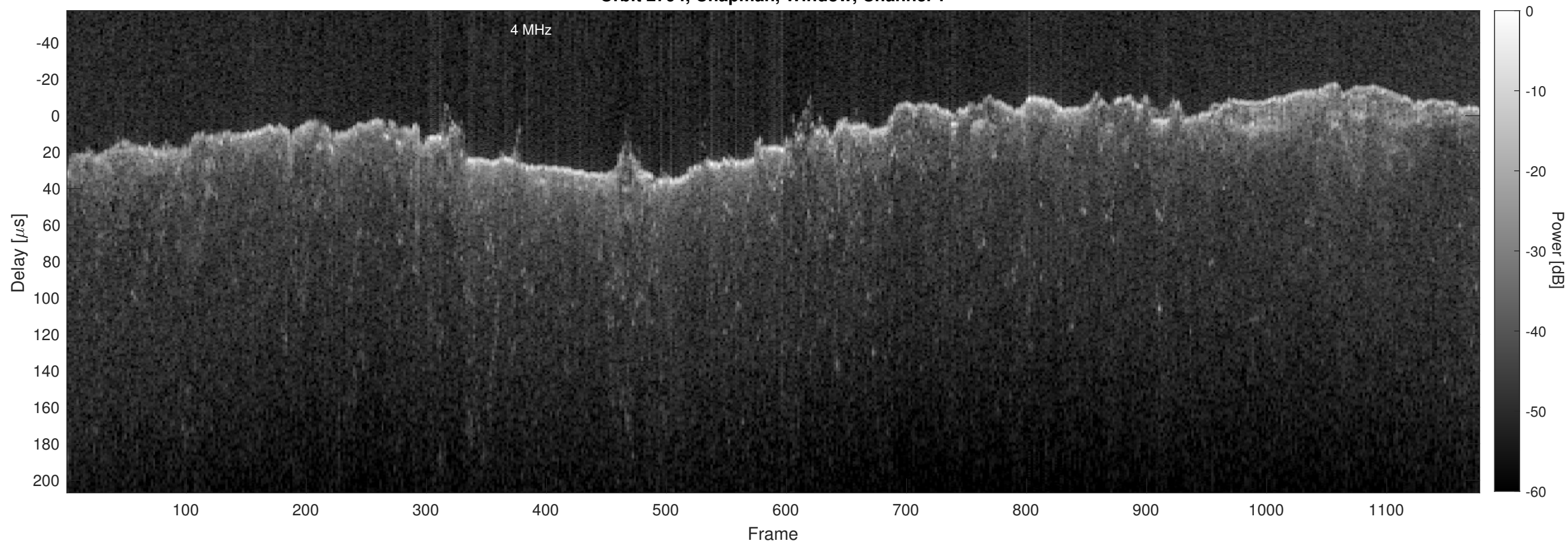
Orbit 2794, Chapman, Window, Channel 2
