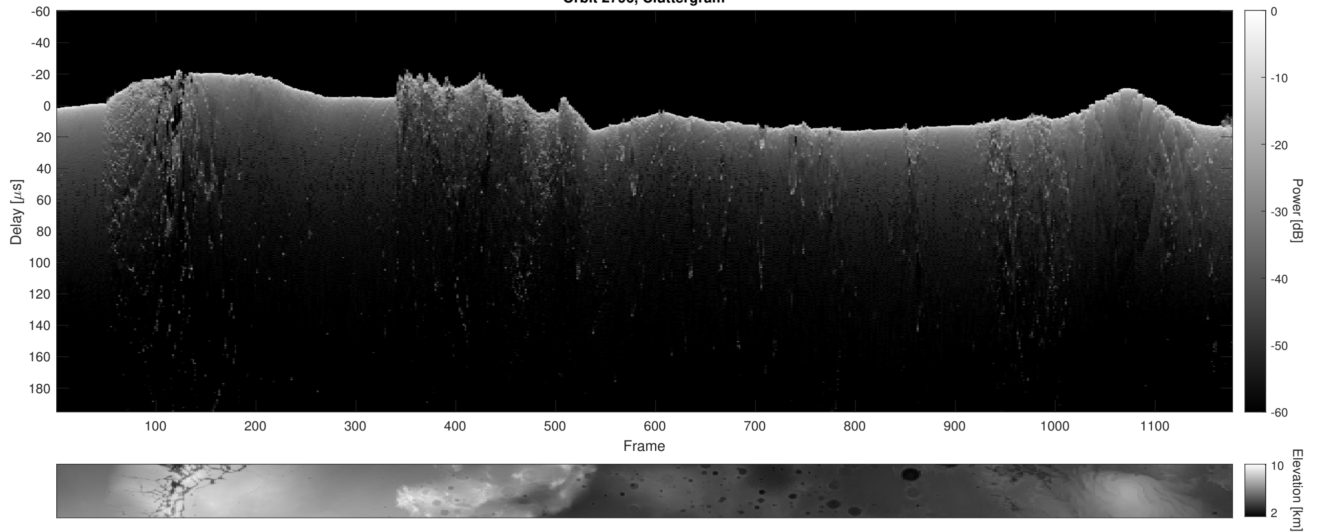
Orbit 2796, Cluttergram
