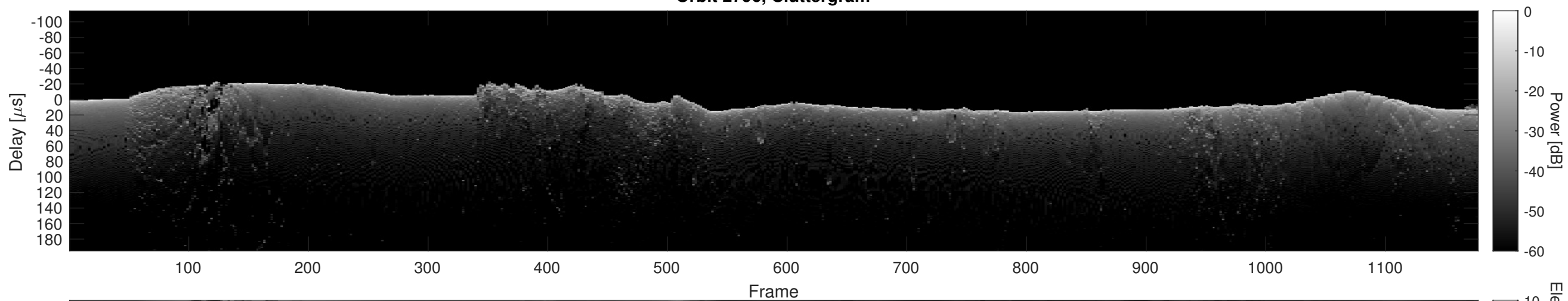
Orbit 2796, Cluttergram
