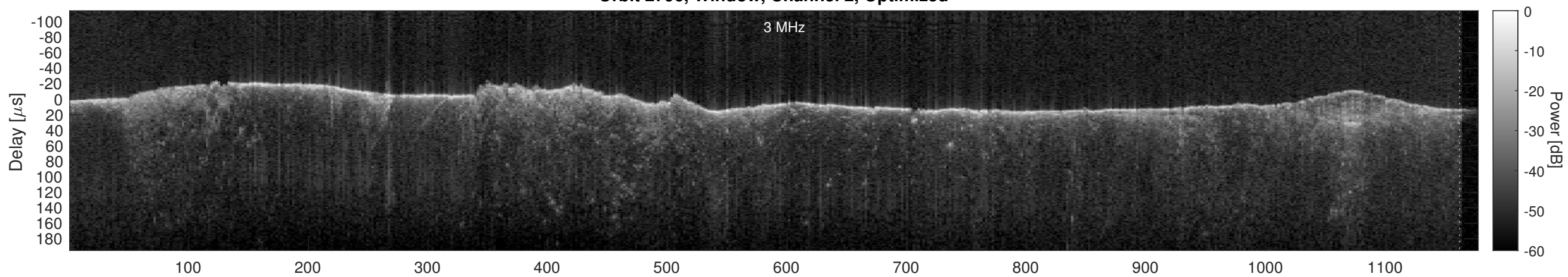
Orbit 2796, Cluttergram
