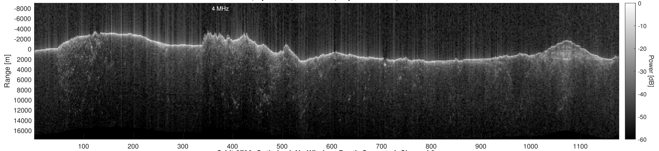
Orbit 2796, Optimized, No Window, Depth-Corrected, Channel 2
