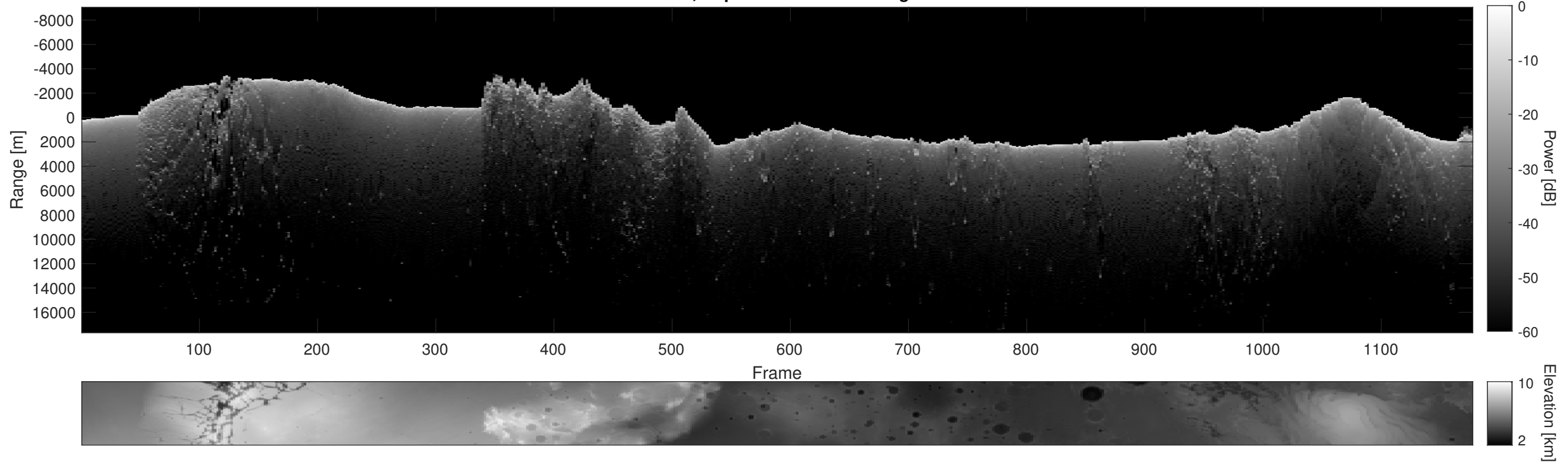
Orbit 2796, Depth-Corrected Cluttergram
