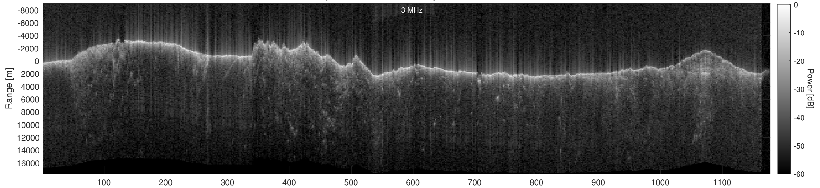
Orbit 2796, Depth-Corrected Cluttergram
