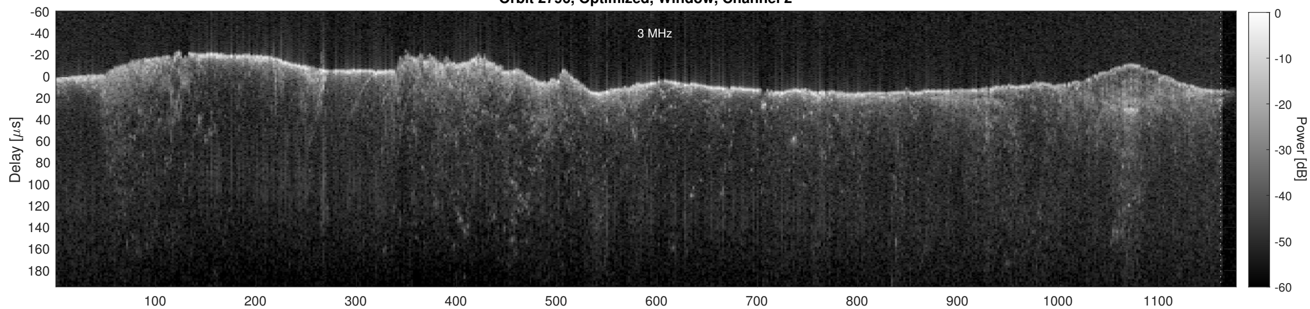
Orbit 2796, Cluttergram
