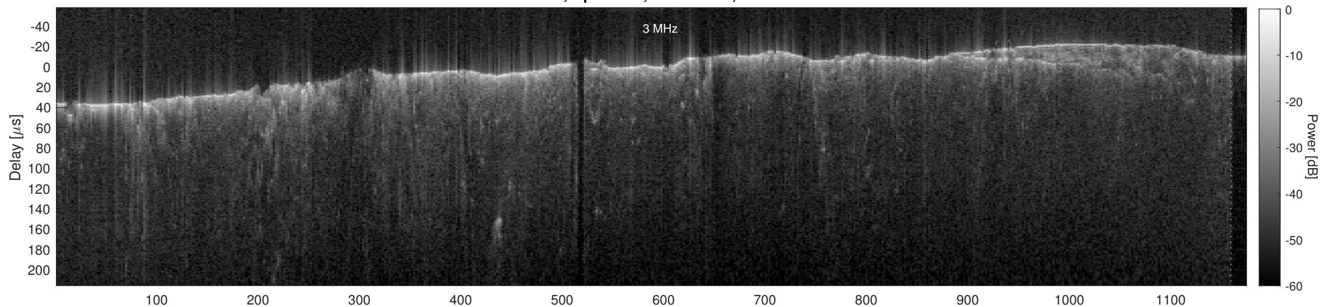
Orbit 2797, Cluttergram
