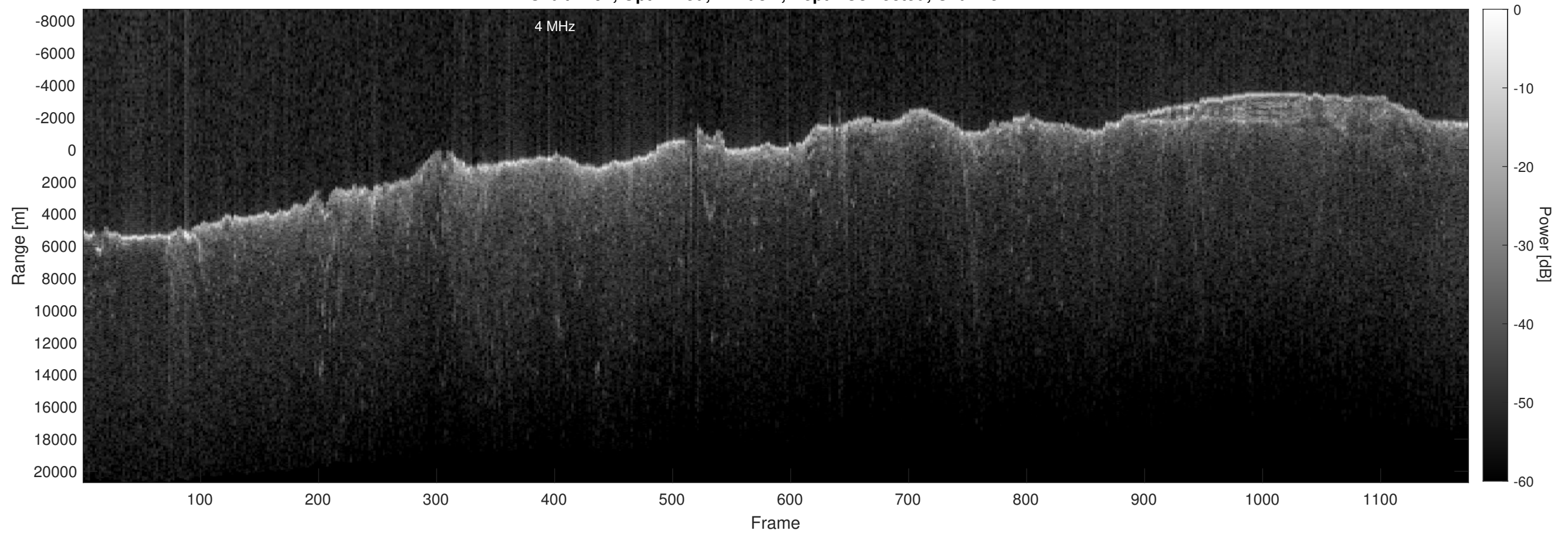
Orbit 2797, Optimized, Window, Depth-Corrected, Channel 2
