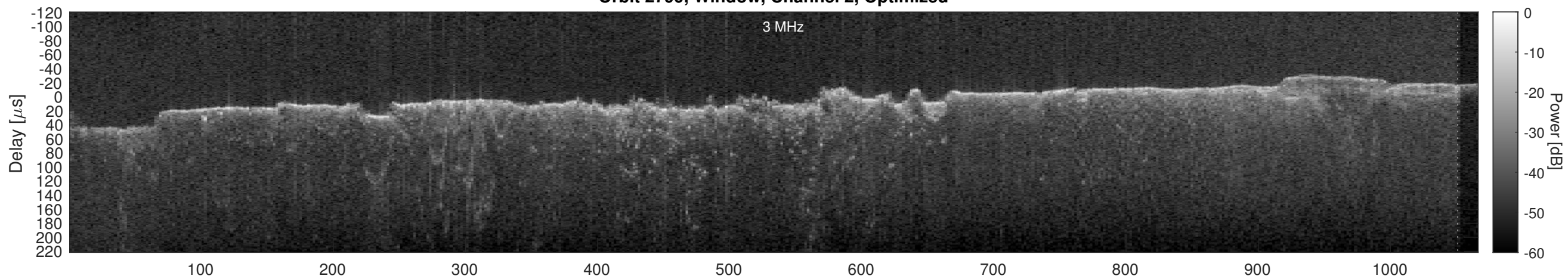
Orbit 2799, Cluttergram
