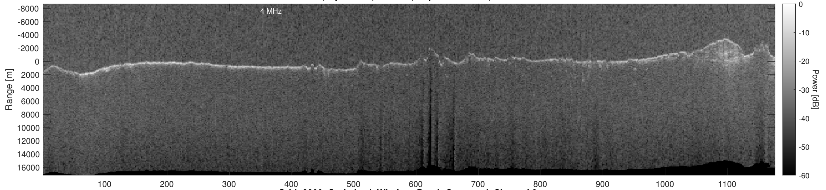
Orbit 2800, Optimized, Window, Depth-Corrected, Channel 2
