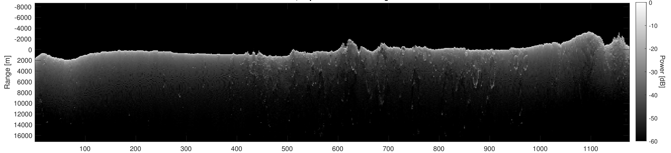
Orbit 2800, Depth-Corrected Cluttergram
