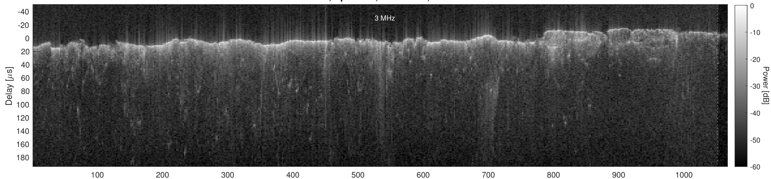
Orbit 2801, Cluttergram
