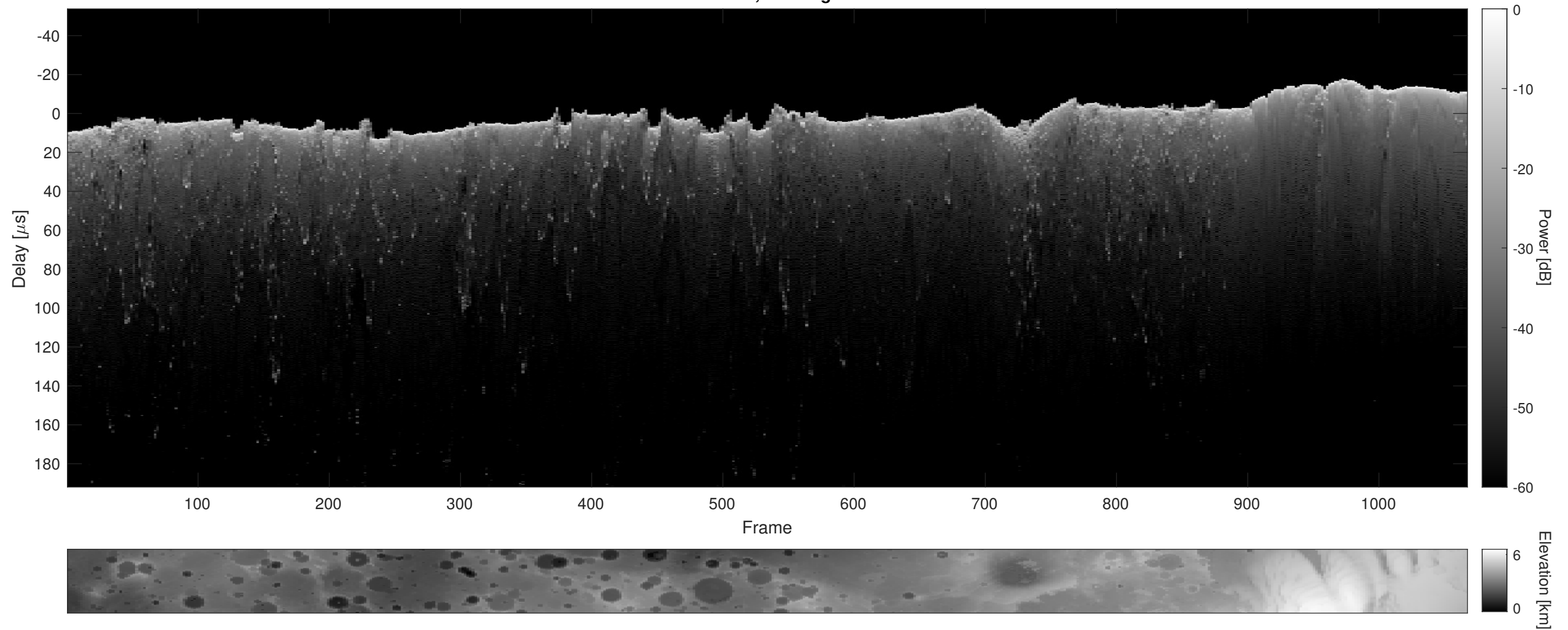
Orbit 2802, Cluttergram
