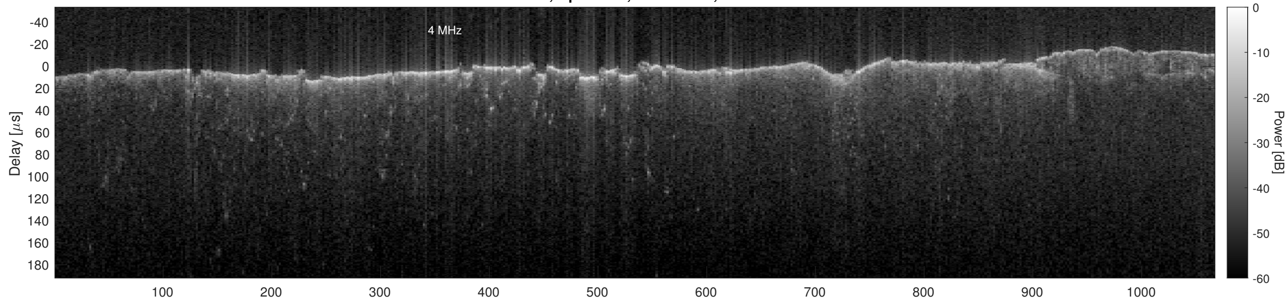
Orbit 2802, Optimized, No Window, Channel 2
