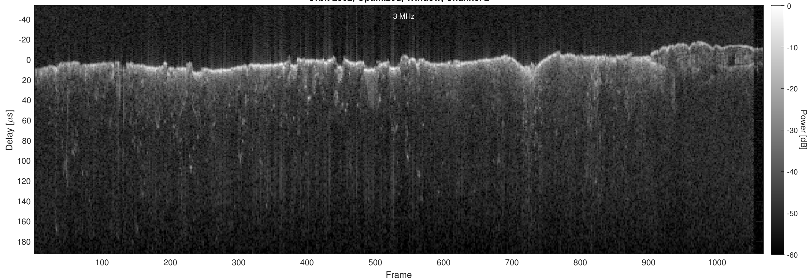
Orbit 2802, Optimized, Window, Channel 2
