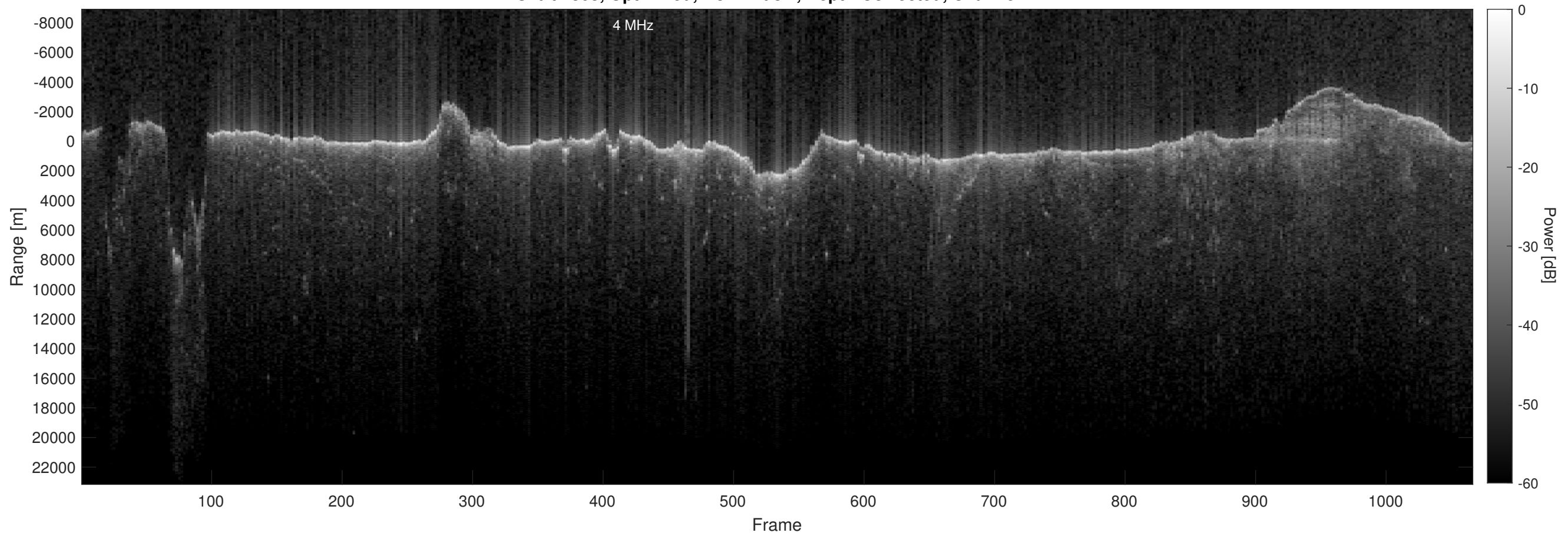
Orbit 2803, Optimized, No Window, Depth-Corrected, Channel 2
