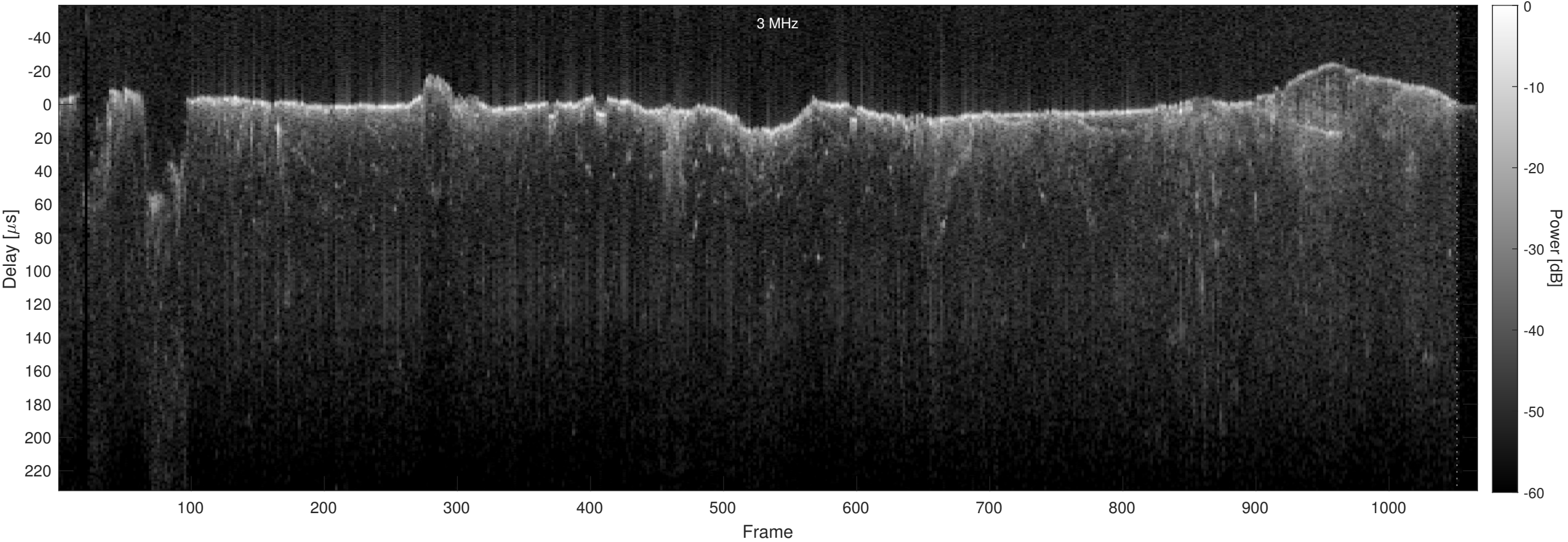
Orbit 2803, Optimized, Window, Channel 2
